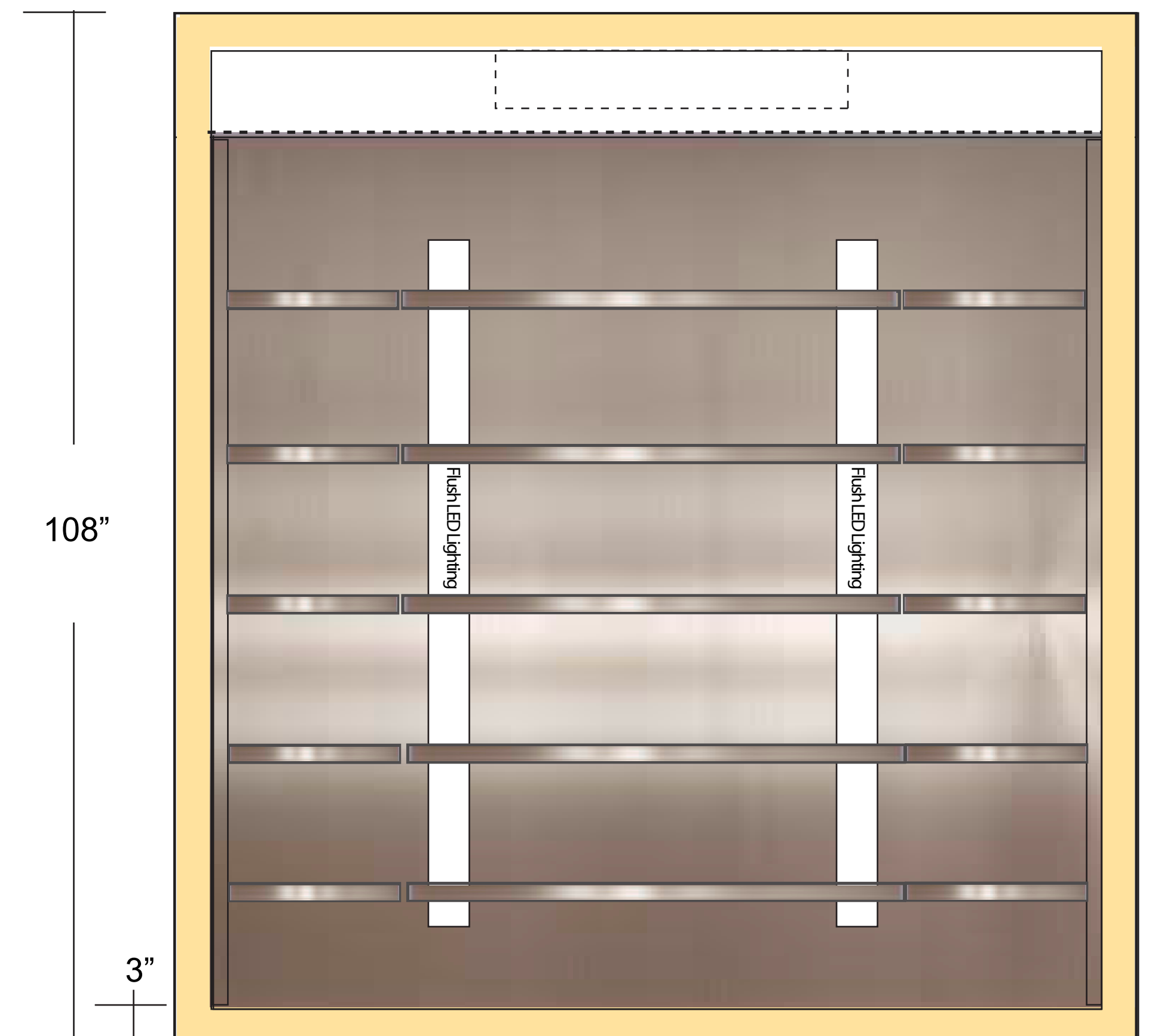
TYPICAL INTERIOR WALL ELEVATION
