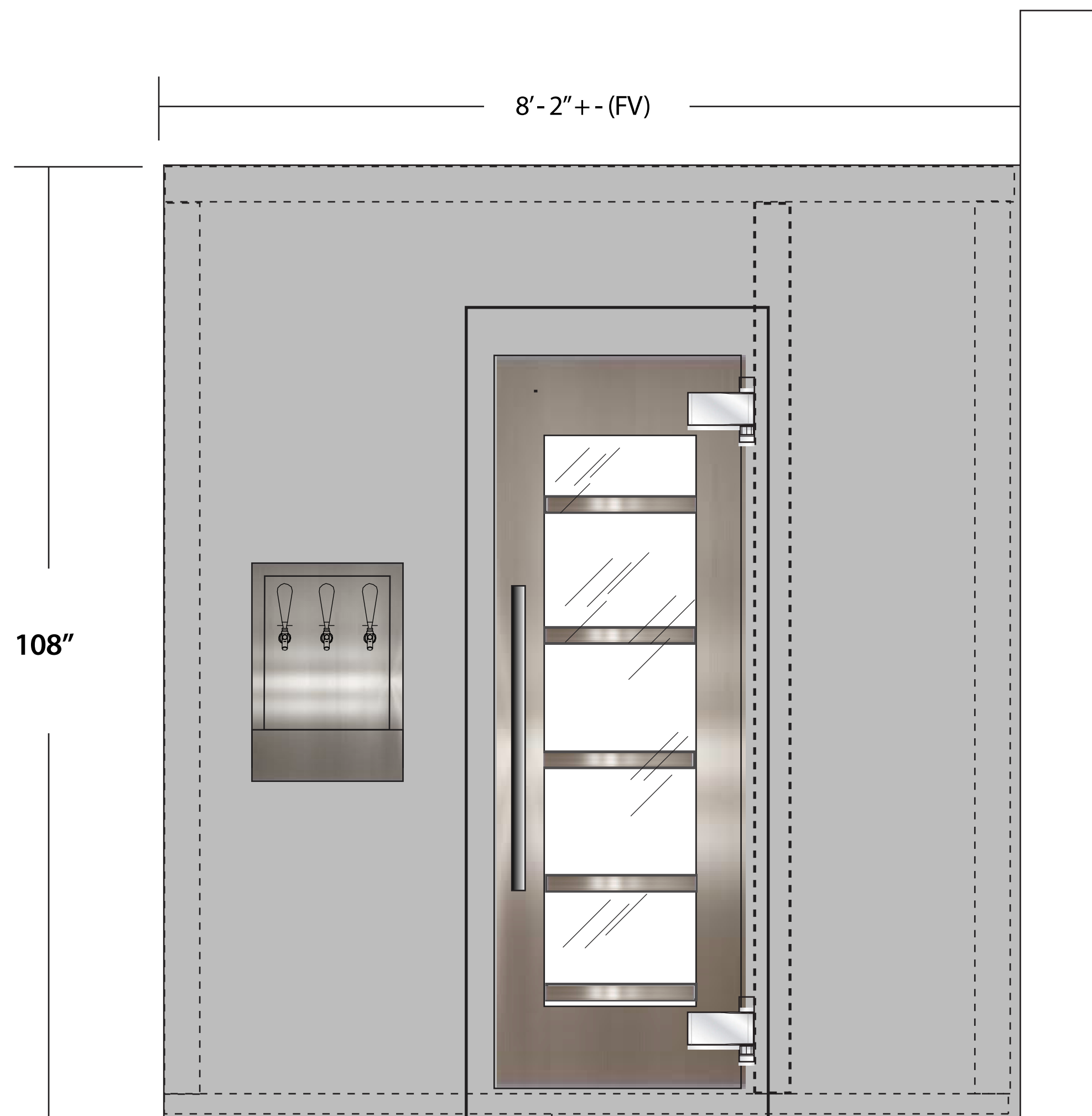
ELEVATION IN BUTLER PANTRY
